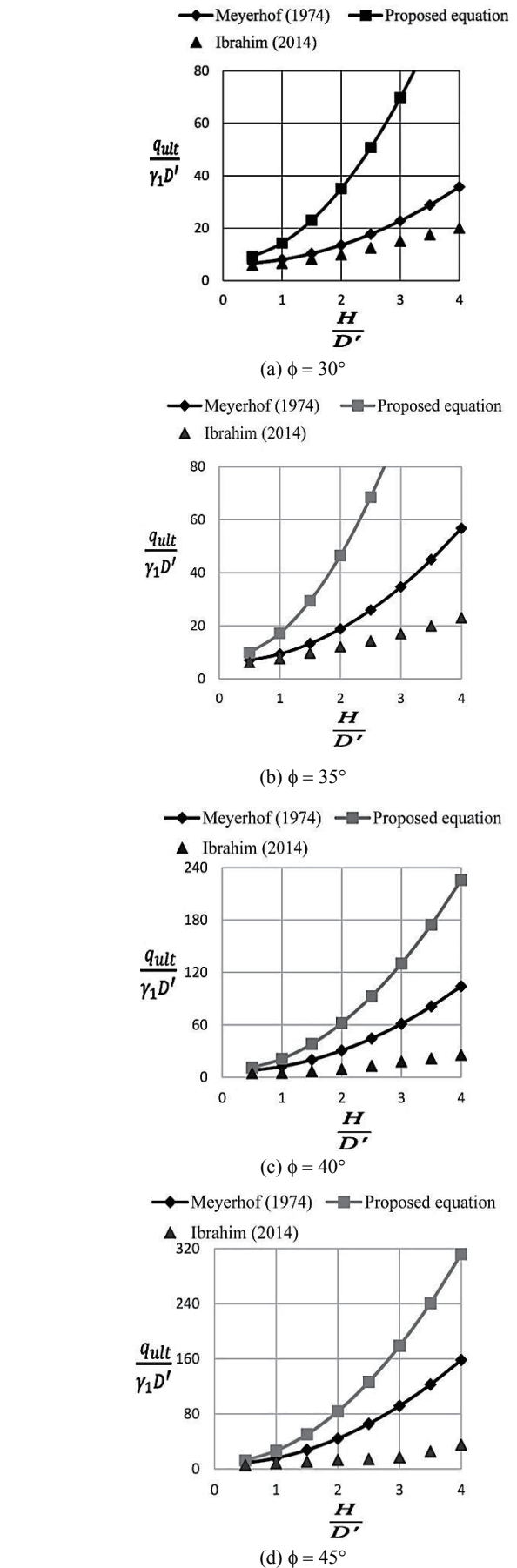
Fig. 6 Plot depicting the variation of q_{ult} / \gamma_1 D' with H/D' when c/\gamma_1 D' = 1.0 , \alpha = 0^\circ , \delta = \phi and D/D' = 0
